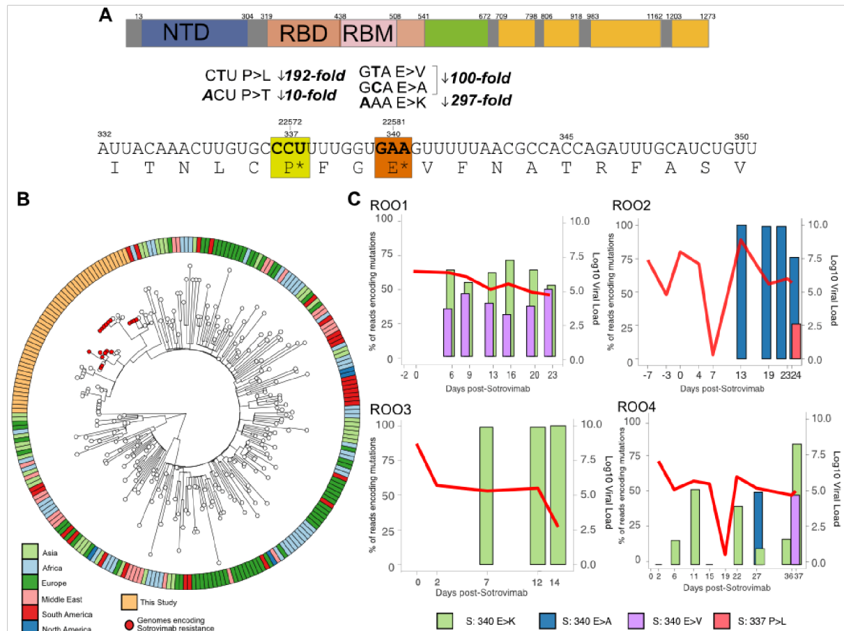
Figure 1. SARS-CoV-2 viral load dynamics and acquisition of resistant mutations following sotrovimab treatment.
